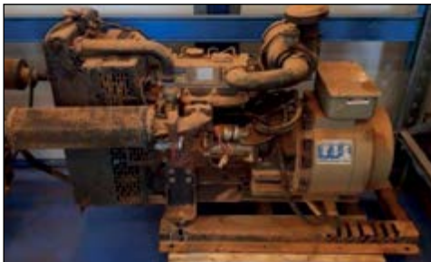
2010 Kubota D1403BG 13 Kva Engine & Generator Suitable for 3 Phase
